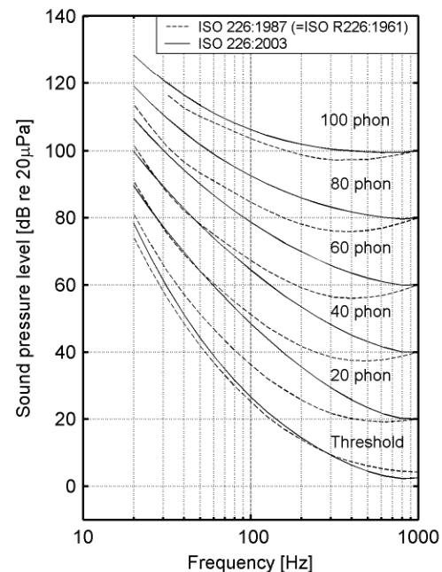
Figure 19. Standardized equal-loudness-level contours.
